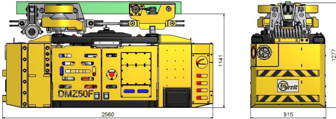
DMZ50F-1 (with one drive)
