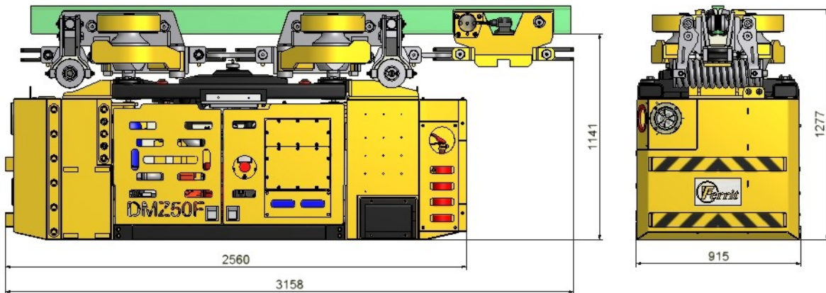
DMZ50F -2 ( with two drives)
